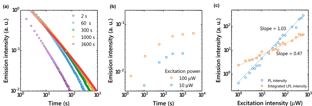
Fig. 3 (a) Emission decay profiles showing the dependence of LPL on the excitation time (1 molar ratio of the donor; excitation power, 100 \mu\text{W} ; temperature, 300 K). (b) Excitation-time dependence of the emission intensity 100 s after photoexcitation. (c) Excitation-power dependence of the emission intensity under photoexcitation (PL) and integrated LPL intensity. The LPL intensity was integrated from 100 s to 10 000 s after photoexcitation. The solid lines show linear fitting.
