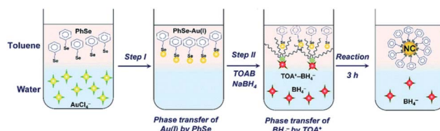
Fig. 3 Schematic diagram of the two-phase synthesis of Au NCs. Reproduced with permission. 27 Copyright 2020 The Royal Society of Chemistry.
