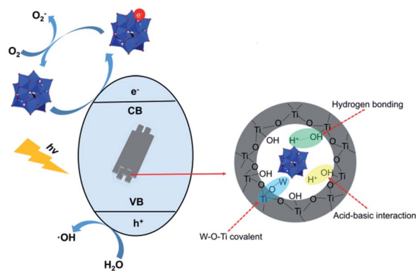
Fig. 4 Structure and photocatalytic mechanism of the H_3PW_{12}O_{40}/TiO_2 composite material. 74
