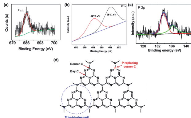
Fig. 1 (a) F 1s XPS spectrum of F/g-CN. Reprinted with permission from ref. 31, copyright 2010, American Chemical Society. (b) F 1s XPS spectrum of F/g-CN. Reprinted with permission from ref. 32, copyright 2018, Elsevier. (c) P 2p XPS spectrum of P/g-CN and (d) illustration of replacement of corner C by P. Reprinted with permission from ref. 33, copyright 2018, Elsevier.
