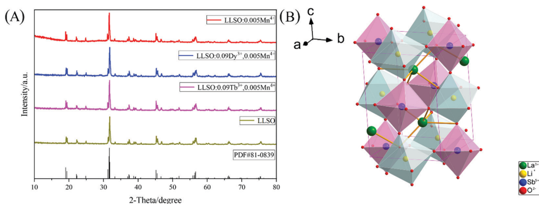
Fig. 1 (A) XRD patterns of \text{LLSO}:\text{0.005Mn}^{4+} ; \text{LLSO}:\text{0.09Tb}^{3+},\text{0.005Mn}^{4+} ; \text{LLSO}:\text{0.09Dy}^{3+},\text{0.005Mn}^{4+} and \text{LLSO} host. (B) Crystal structure schematic diagram of \text{La}_2\text{LiSbO}_6 .
