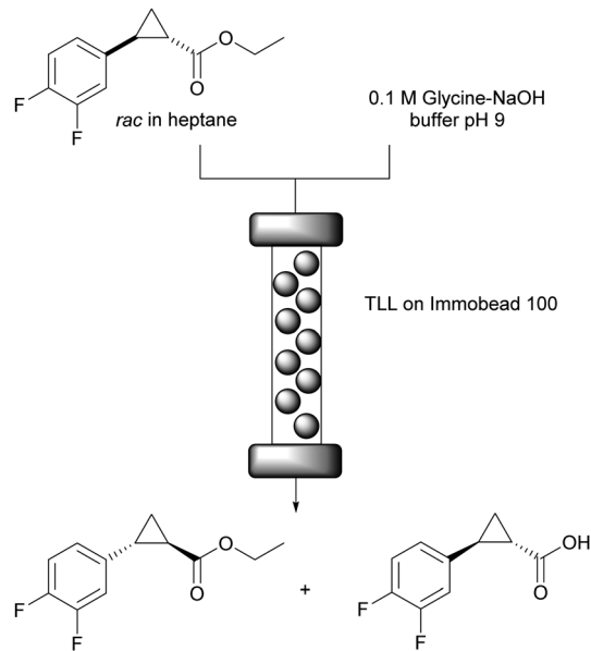
Fig. 5 TLL catalyzed kinetic resolution of rac -cyclopropanecarboxylate ester yielding (1 S ,2 S )-2-(3,4-difluorophenyl) cyclopropan-1-amine. The unaltered (1 R ,2 R ) ester is converted into the desired amine.
