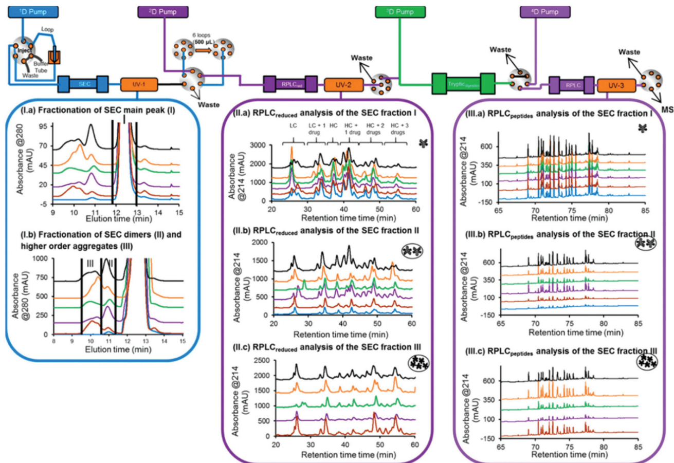
Fig. 5 Schematic representation of an automated 4D-LC-MS workflow for SEC coupled to online peptide mapping, enabling the separation and fractionation of size variants by SEC ( ^1\text{D} ) followed by on-column reduction by RPLC ( ^2\text{D} ), trypsin digestion in flow-through mode ( ^3\text{D} ), and peptide mapping analysis by RPLC ( ^4\text{D} ). (I, a, b) SEC of ADC product reference, and samples stressed thermally, by light, at basic pH, at acidic pH, and under oxidative conditions (blue, brown, purple, green, orange, gray, and black traces, respectively). (II, a–c) ^2\text{D} RPLC of the SEC heart-cut fractions that have been reduced online and then eluted. (III, a–c) ^4\text{D} RPLC of the SEC heart-cut fractions that have been reduced and trypsin digested online. Reproduced from A. Goyon, M. Kim, L. Dai, C. Cornell, F. Jacobson, D. Guillarme, et al., Streamlined Characterization of an Antibody–Drug Conjugate by Two-Dimensional and Four-Dimensional Liquid Chromatography/Mass Spectrometry, Anal. Chem. , 2019, 91, 2314896–14903. With permission from American Chemical Society, copyright 2019.
