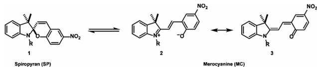
Fig. 2 Typical structural formula of a spiroindolinopyran.
