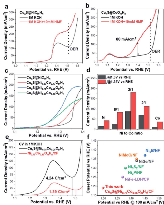
Fig. 2 (a and b) LSV curves of \text{Cu}_x\text{S}@NiO_mH_n and \text{Cu}_x\text{S}@CoO_mH_n towards electrochemical HMF oxidation. (c) Comparison of LSV curves of prepared electrodes at 1.3 V and 1.35 V vs. RHE. (d) Current densities of prepared electrodes at 1.3 V and 1.35 V vs. RHE. (e) CV curves of \text{Cu}_x\text{S}@Ni_{0.75}Co_{0.25}O_mH_n , Ni_{0.75}Co_{0.25}O_mH_n/CF in 1 M KOH and calculated charges for the oxidation of transition metal cations prior to the oxygen evolution reaction. (f) Performance comparison of \text{Cu}_x\text{S}@Ni_{0.75}Co_{0.25}O_mH_n with reported electrocatalysts towards electrochemical oxidation of HMF, urea and primary amine.
