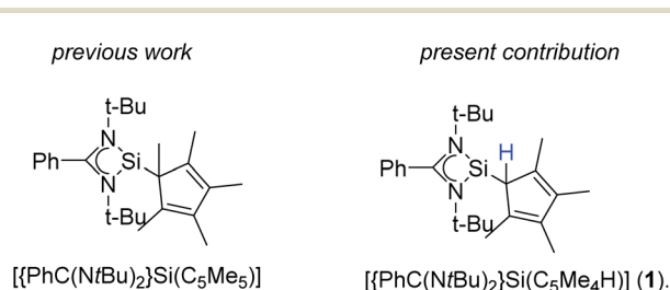
Scheme 1 Comparison of the previous and herein published silylene.
