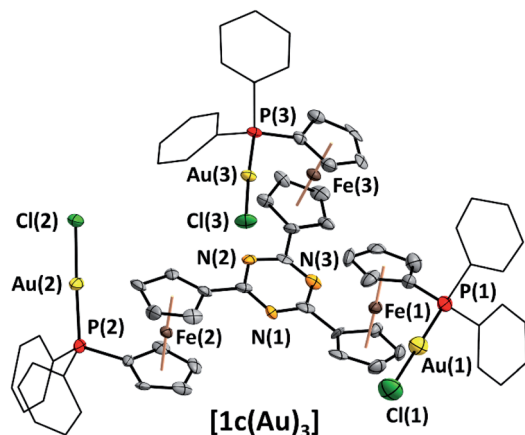
Fig. 2 Molecular structure of homotrimeric [1c(\text{Au})_3] with partial atom numbering scheme. Thermal ellipsoids are set at the 50% probability level. For clarity, the phenyl rings are depicted in wireframe style, and co-crystallised solvent, disorder in the P(2)–Au(2)–Cl(2) fragment, and hydrogen atoms have been omitted.
