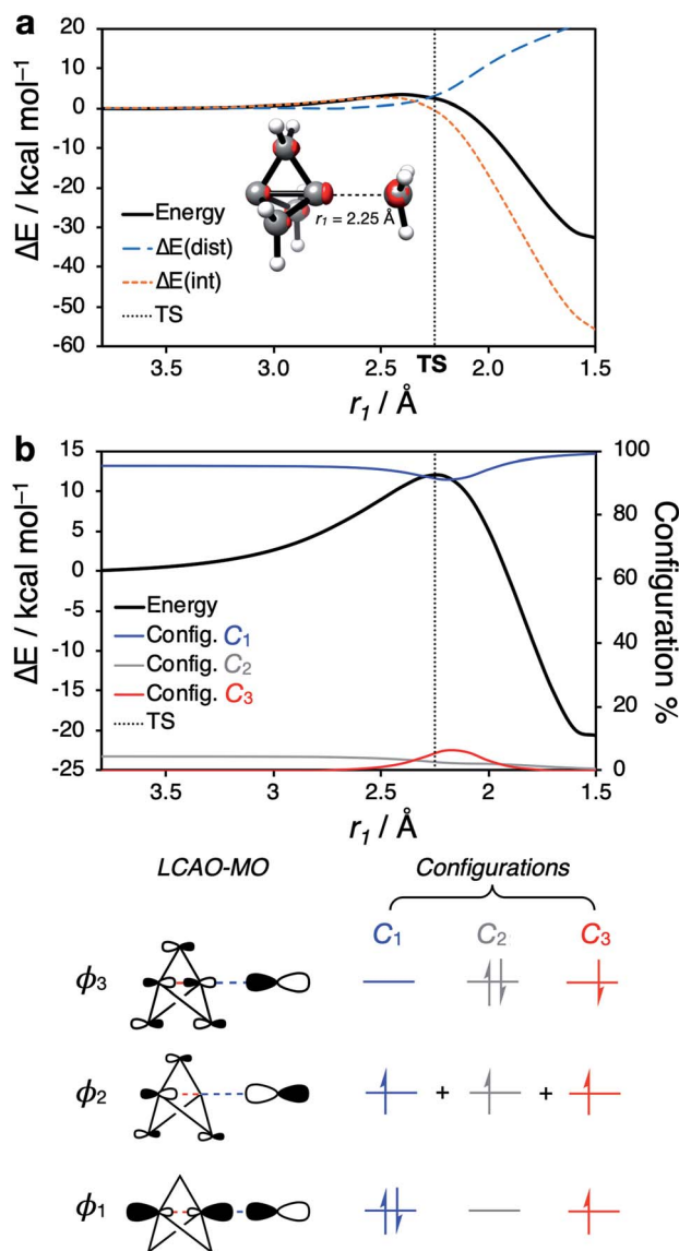
Fig. 5 (a) PES (DLPNO-CCSD(T)/def2-QZVPP//CASSCF(3,3)/def2-QZVPP) and distortion/interaction energies for the addition of \cdot\text{CH}_3 to 1. (b) (Top) PES (CASSCF(3,3)/def2-QZVPP) for the addition of a methyl radical to 1, showing the proportion of each leading electronic configuration as a function of the forming C-C bond ( r_1 ). (Bottom) LCAO-MO depiction of the frontier molecular orbitals involved in the radical addition process to 1, and the leading electronic configurations for the reaction.
