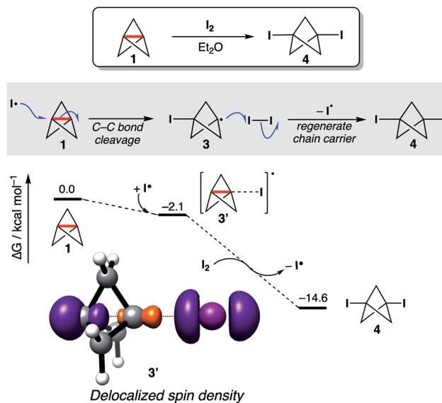
Fig. 6 Proposed mechanism for the diiodination of 1 (top), and free energy profile for the diiodination of 1, calculated at SMD( \text{Et}_2\text{O} )-DLPNO-CCSD(T)/def2-QZVPP//SMD( \text{Et}_2\text{O} )-B2GP-PLYP-D3BJ/def2-TZVP. Spin density of 3' is plotted at an isovalue of 0.01 a.u.
