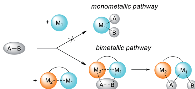
Scheme 1 Schematic representation of the altering reactivity of a single metal center through heterobimetallic complex formation.
