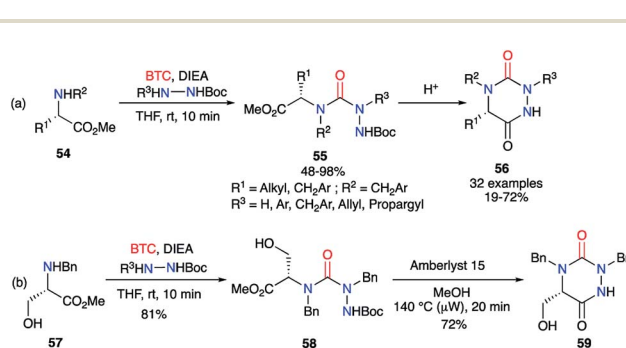
Scheme 20 (a) Aza-DKPs synthesis from enantiopure amino acids; (b) aza-DKP synthesis from the unprotected L -serine.
