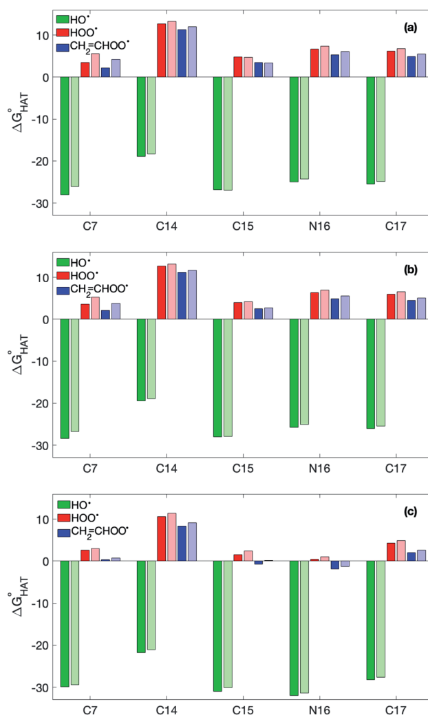
Fig. 3 \Delta G_{\text{HAT}} ( \text{kcal mol}^{-1} ) in the gas phase (a), in benzene (b), and in water (c) for the scavenging of \text{HO}^\bullet , \text{HOO}^\bullet and \text{CH}_2=\text{CHOO}^\bullet from non-aromatic sites of selenofluoxetine. Values for fluoxetine taken from Muraro et al. 17 are showed in a lighter shade for comparison. Level of theory: (SMD)-M06-2X/6-311+G(d,p)//M06-2X/6-31G(d).
