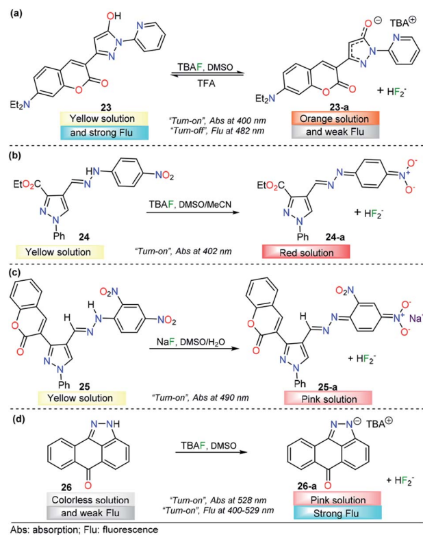
Fig. 13 Probes for \text{F}^- ions based on the pyrazole derivatives (a) 23 , (b) 24 , (c) 25 , and (d) 26 .
