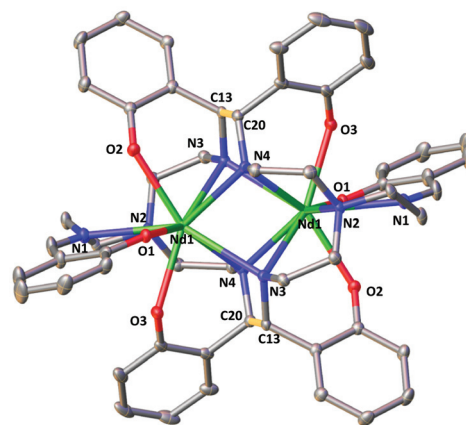
Fig. 3 Molecular structure of complex 4-Nd (C–C bonds between imino highlighted in yellow, 50% probability ellipsoids Hydrogen atoms, potassium atoms and THF molecules were omitted for clarity).
