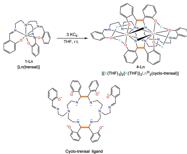
Scheme 4 Synthesis of [K(THF) 3 ] 2 (K(THF) 2 ) 2 Ln 2 (cyclo-trensal)], 4-Ln , Ln = Nd, Sm.
