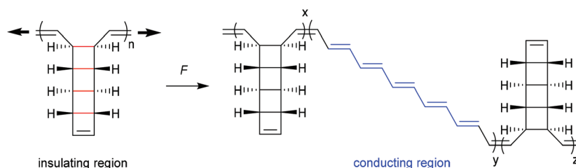
Scheme 13 Mechanical unzipping of polyadderenes.
