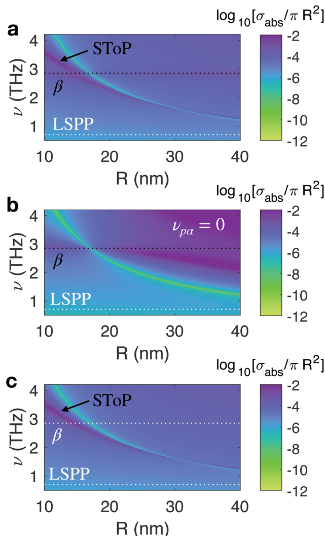
Fig. 6 Modifying the dielectric function: (a) Absorption cross-section with LSP mode (highlighted with white dotted line) removed from the dielectric function ( \nu_{p,f} = 0 ). (b) Absorption cross-section with both LSP and \alpha phonon contributions removed ( \nu_{p,f} = \nu_{p,\alpha} = 0 ). The trough of zero-absorption is still seen, but the SToP mode is no longer present. (c) Absorption cross-section with both LSP and \beta phonon contributions (highlighted with a white dotted line) removed ( \nu_{p,f} = \nu_{p,\beta} = 0 ).
