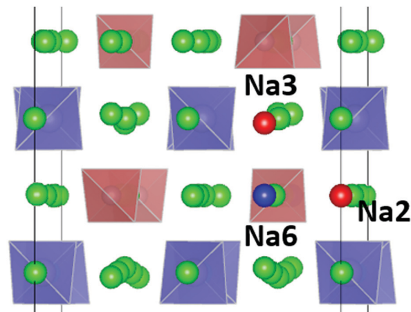
Fig. 11 Snapshot of a configuration with an occupied Na6 site (blue sphere). Occupying the Na6 site is only possible, if two of the 6 neighbouring sites (4 Na2 or 2 Na3) sites are vacant. Red spheres indicate these vacancies (here 1 on Na2 and 1 on a Na3 site).
