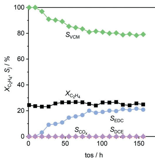
Fig. 10 Conversion and selectivity as a function of time-on-stream in ethene oxychlorination over a CeO_2/ZrO_2-Ca-I/Al_2O_3 system as depicted in the fourth panel of Fig. 9. Conditions are detailed in Table 2.
