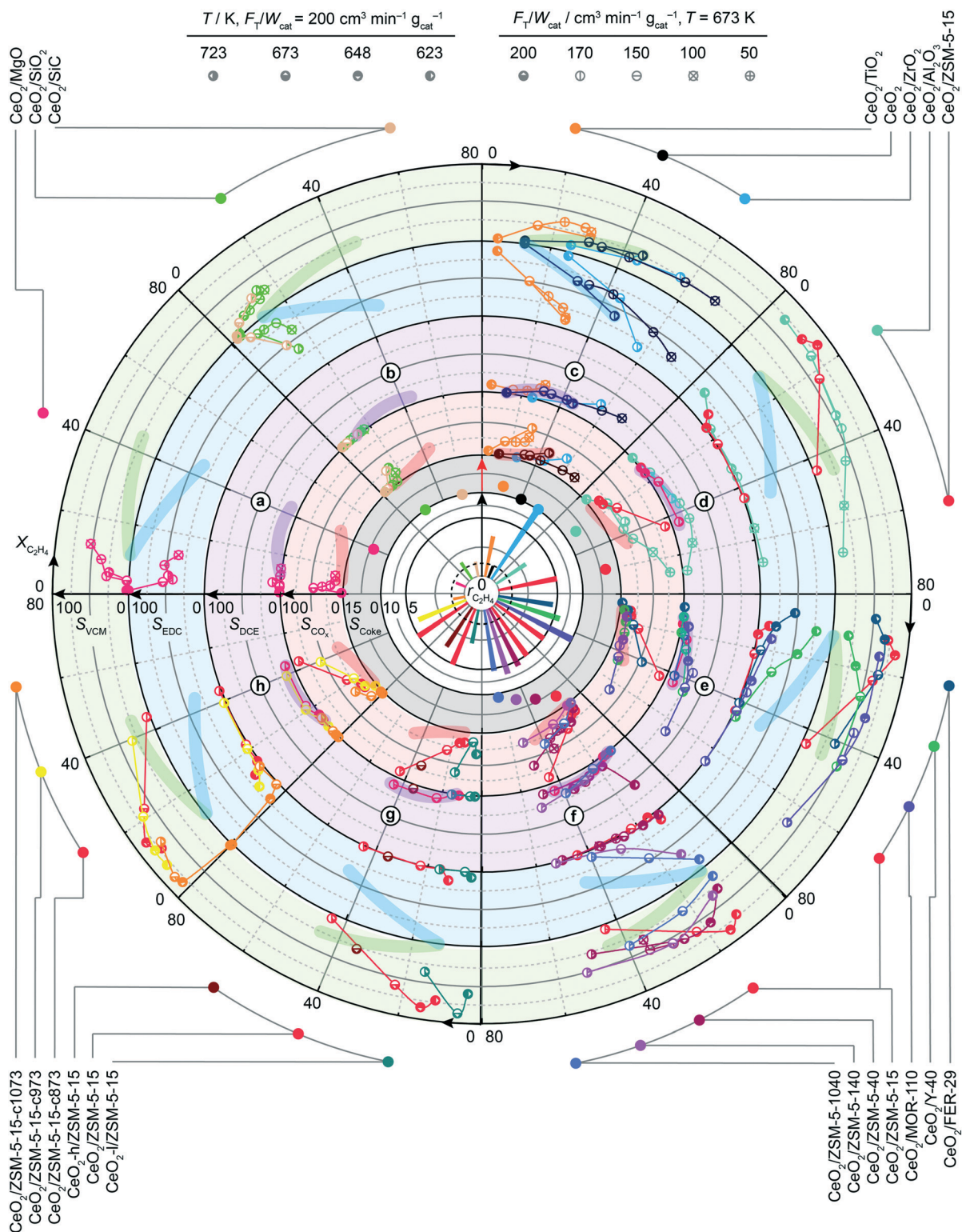
Fig. 3 Reaction rates (in \text{mol h}^{-1} \text{mol}_{\text{C}_2\text{H}_4}^{-1} ) and coke selectivity (in %) at 673 K, and product selectivities (in %) recorded as a function of ethene conversion (in %) for ceria catalysts supported over a)–d) different carriers, and e)–h) zeolite supports, with various framework types, Si:Al ratios, Ce-loading, and calcination temperatures, respectively. The catalysts are identified by a colour code, indicated on the outside of the circle, while catalytic data points were recorded using the conditions that are specified by the symbol interior, as indicated at the top. The performance of bulk CeO 2 is used as a benchmark, indicated by the dashed circle and highlighted regions. Conditions are detailed in Table 2.
