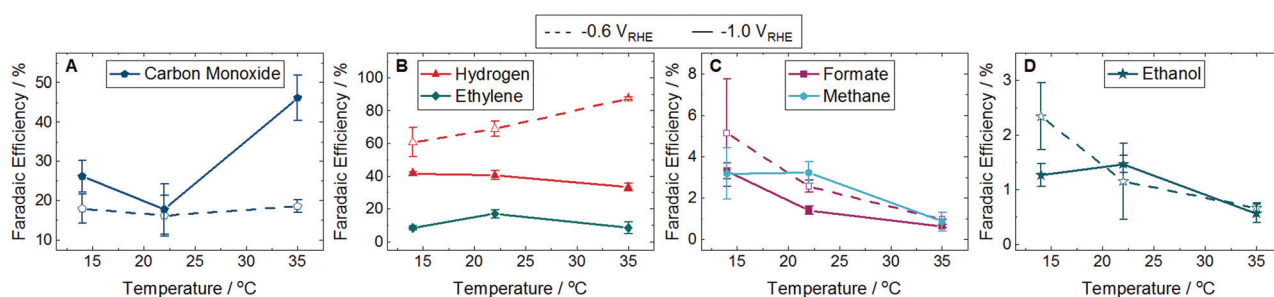
Fig. 3 Faradaic efficiency (FE) of major products at 14, 22, and 35 °C in the dark. Dashed lines with unfilled symbols show results performed at -0.6 V_{\text{RHE}} and solid lines with filled symbols show results performed at -1.0 V_{\text{RHE}} . Products shown are (A) carbon monoxide, (B) hydrogen and ethylene, (C) formate and methane, and (D) ethanol. Fig. S14 in the ESI † shows the partial current densities for these major products. Ethylene and methane were not detected at any temperature at -0.6 V_{\text{RHE}} . The FE and partial current densities of the minority products methanol, glycolaldehyde, acetaldehyde, ethane, hydroxyacetone, acetone, allyl alcohol, propionaldehyde, and n -propanol are shown in Fig. S15 and S16 in the ESI † , respectively. Error bars represent one standard deviation of experiments performed in triplicate.
