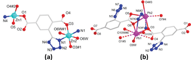
Fig. 1 Coordination environments of the Zn(II) ions and Pb(II) ions in 1 (a) and 2 (b); symmetry codes for 1 : #1: 2-x, 1-y, 1-z and #2: 1.5-x, 0.5+y, 0.5-z ; for 2 : #1: 1-x, 1-y, 1-z ; #2: -x, -y, 2-z ; #3: x-1, y, z ; #4: x, 1+y, z ; #5: x, y-1, z ; and #6: 1-x, -y, 2-z .
