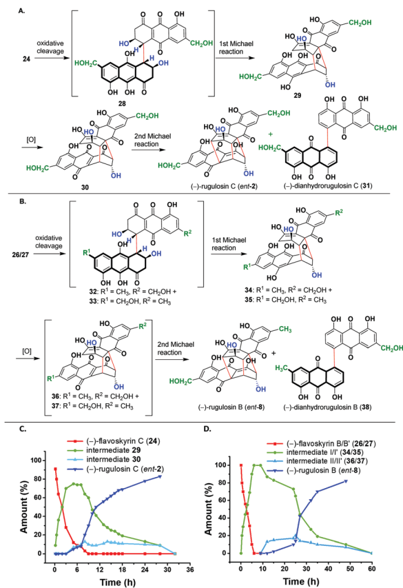
Scheme 4 (A) Cascade conversion of (-)-flavoskyrin C (24) to (-)-rugulosin C ( ent -2). (B) Cascade conversion of (-)-flavoskyrin B/B' (26/27) to (-)-rugulosin B ( ent -8). (C) Plot of percentage conversion of the products formed with time (h) for the cascade in (A). (D) Plot of percentage conversion of the products formed with time (h) for the cascade in (B).
