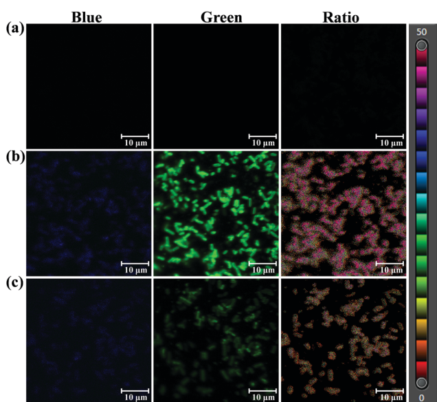
Fig. 4 Confocal microscopic images of Escherichia coli incubated with PNA ( 50 \mu\text{M} ). (a) Blank group. (b) Escherichia coli -PGA + with PGA high expression. (c) Escherichia coli -PGA + incubated with the inhibitor oleanolic acid ( 50 \mu\text{M} ). Blue channel: \lambda_{\text{ex}} 405/\lambda_{\text{em}} 425\text{--}459 \text{ nm} , green channel: \lambda_{\text{ex}} 405/\lambda_{\text{em}} 525\text{--}575 \text{ nm} . Scale bar 10 \mu\text{m} .
