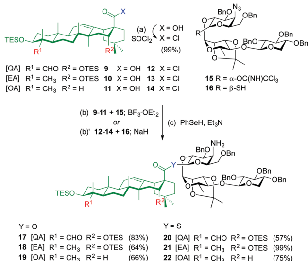
Scheme 1 Reagent and conditions: (a) \text{SOCl}_2 , Py, DCM, 0 °C to r.t., 2 h, 99%; (b) \text{BF}_3 \cdot \text{Et}_2\text{O} , 4 Å MS, DCM, −78 °C, 6 h (b') NaH, THF, 0 °C to r.t., 3 h; (c) \text{PhSeH} , \text{Et}_3\text{N}/\text{THF}/\text{toluene} 10 : 3 : 3, 40 °C, 3 h, 83% (2 steps) (for 17 ), 64% (2 steps) (for 18 ), 66% (2 steps) (for 19 ); 57% (2 steps) (for 20 ), 99% (2 steps) (for 21 ), 75% (2 steps) (for 22 ).
