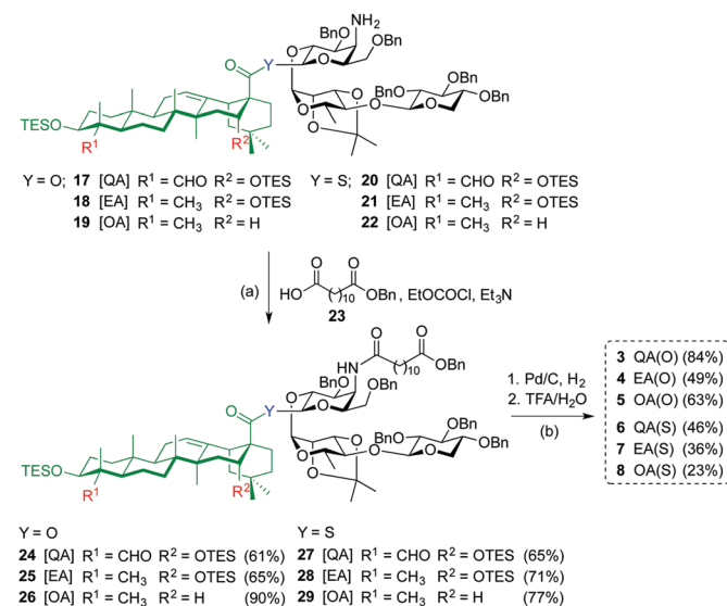
Scheme 2 Reagent and conditions: (a) \text{EtOCOC}_9\text{OBn} , \text{Et}_3\text{N} , THF, 0 °C to r.t., 4 h, 61% (for 24 ), 65% (for 25 ), 90% (for 26 ); 65% (for 27 ), 71% (for 28 ), and 77% (for 29 ); (b) 1: Pd/C, \text{H}_2 (1 atm), \text{EtOH}/\text{THF} 1 : 1, r.t., 16 h (for 24–26 ); 20 min (for 27–29 ); 2: TFA/ \text{H}_2\text{O} 3 : 1, 0 °C, 1 h, 84% (for 3 ), 49% (for 4 ), 63% (for 5 ); 46% (for 6 ), 36% (for 7 ), and 23% (for 8 ).
