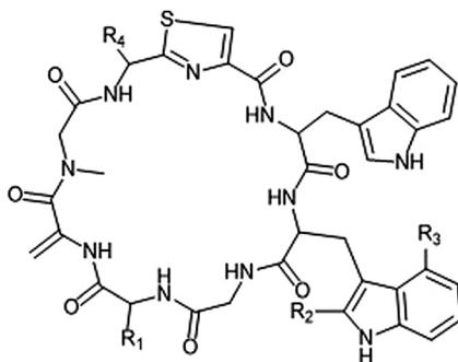
Argyrin A (30): R_1 = \text{CH}_3 , R_2 = \text{H} Argyrin C (32): R_1 = \text{CH}_3 , R_2 = \text{CH}_3 R_3 = \text{OCH}_3 , R_4 = \text{CH}_3 Argyrin B (31): R_1 = \text{CH}_2\text{CH}_3 , R_2 = \text{H} Argyrin D (33): R_1 = \text{CH}_2\text{CH}_3 , R_2 = \text{CH}_3 R_3 = \text{OCH}_3 , R_4 = \text{CH}_3 Argyrin F (34): R_1 = \text{CH}_3 , R_2 = \text{H} R_3 = \text{OCH}_3 , R_4 = \text{CH}_2\text{OH}
