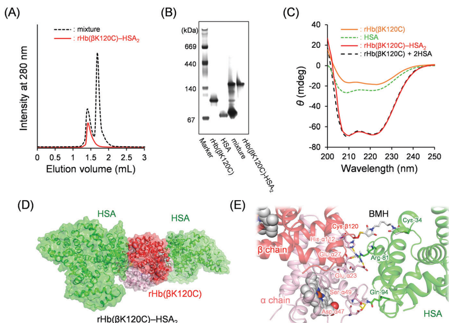
Fig. 3 (A) SEC profiles of the resultant reaction mixture [rHb( \beta K120C) + MA-HSA] and the purified rHb( \beta K120C)-HSA 2 trimer. (B) Native PAGE patterns of rHb( \beta K120C), HSA, the reaction mixture, and the purified rHb( \beta K120C)-HSA 2 trimer. (C) CD spectra of rHb( \beta K120C), HSA, rHb( \beta K120C)-HSA, and rHb( \beta K120C)-HSA in PBS at 25 °C ([protein] = 0.2 \mu M). (D and E) The energy-minimized structure of the rHb( \beta K120C)-HSA 2 trimer obtained by a molecular dynamics (MD) calculation using the Desmond software.
