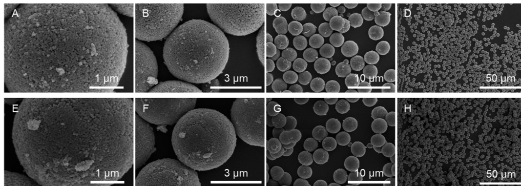
Fig. 2 SEM images of (A–D): bare CaCO 3 particles and (E–H): polymer-modified CaCO 3 -PMAcO particles.
