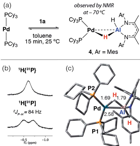
Scheme 2 (a) Reversible reaction of 1a with [\text{Pd}(\text{PCy}_3)_2] . (b) Hydride region of the ^1\text{H} NMR spectrum at -70^\circ\text{C} in toluene- d_8 . (c) Calculated structure of 4 with selected bond lengths in Å.
