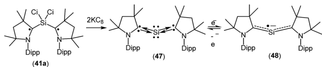
Fig. 13 cAAC-stabilized siladibene and in situ generation of ( {}^{\text{Me}^2\text{cAAC}}\text{Si} ) 2 Si •− .
