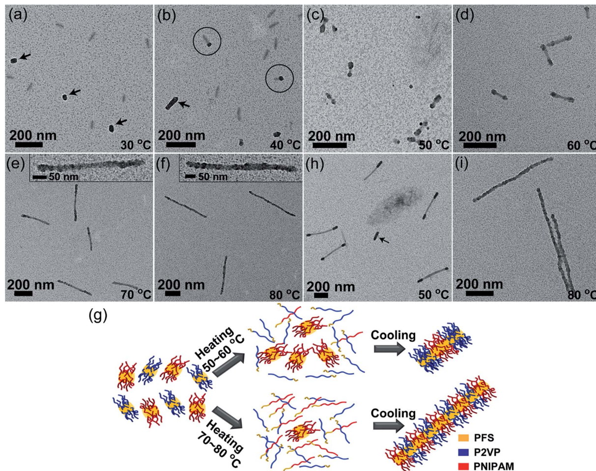
Fig. 4 Self-seeding of a PFS 26 -b-PNIPAM 190 and PFS 17 -b-P2VP 170 fragment mixture (mass ratio 1 : 1). (a–f) TEM images of the micelles obtained by annealing the mixture at 30 to 80 °C. The arrows in (a) indicate the PFS 17 -b-P2VP 170 fragments. The arrow in (b) indicates a PFS 17 -b-P2VP 170 homomicelle. The circles in (b) indicate matchstick-like micelles. The insets in (e and f) show magnified TEM images of patchy comicelles. (g) Schematic diagram of the self-seeding process of the fragment mixture. (h and i) TEM images of the micelles obtained by annealing a mixture of PFS 26 -b-PNIPAM 190 micelles ( L_n = 290 nm) and PFS 17 -b-P2VP 170 fragments ( L_0 = 43 nm) at (h) 50 °C and (i) 80 °C. The arrow in (h) indicates a PFS 17 -b-P2VP 170 homomicelle. The P2VP chains were selectively stained with PtNPs.
