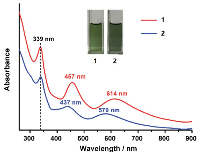
Fig. 4 The optical absorption spectra of [\text{Ag}_{34}(\text{BTCA})_3(\text{C}\equiv\text{CBu})_9(-\text{tfa})_4(\text{CH}_3\text{OH})_3](\text{SbF}_6) (1) and [\text{AuAg}_{33}(\text{BTCA})_3(\text{C}\equiv\text{CBu})_9(-\text{tfa})_4(\text{CH}_3\text{OH})_3](\text{SbF}_6) (2) in dichloromethane solution. Inset: photographs of cluster solutions.
