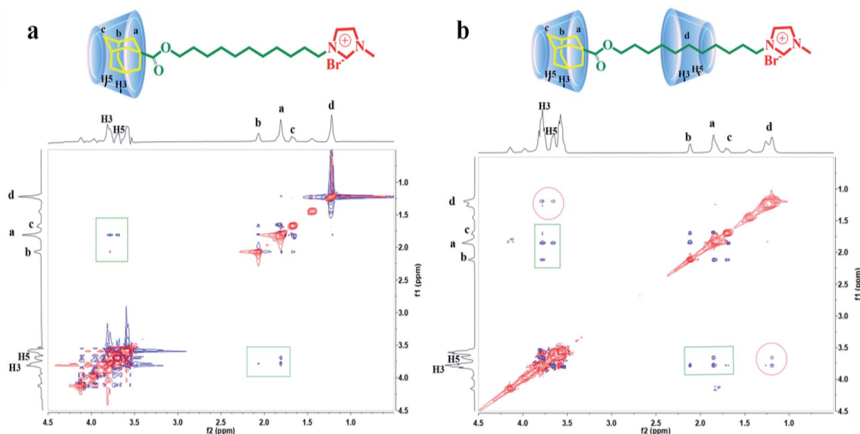
Fig. 5 ^1\text{H} - ^1\text{H} 2D ROESY spectra of 10 mM AD-C 11 im@1 \beta -CD (a) and 10 mM AD-C 11 im@2 \beta -CD (b).
