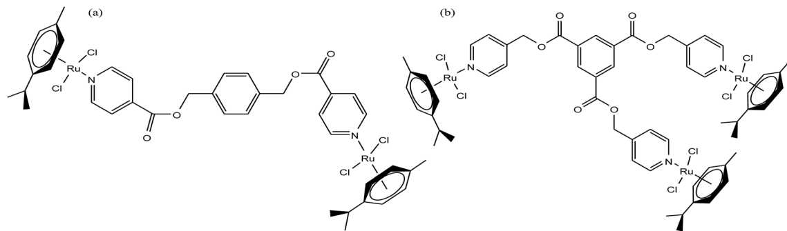
Fig. 3 Chemical structure of (a) dinuclear [\text{Ru}_2(\eta^6\text{-}p\text{-cymene})_2(\text{DIXD})\text{Cl}_2] and (b) trinuclear [\text{Ru}_3(\eta^6\text{-}p\text{-cymene})_3(\text{BTPE})\text{Cl}_6] ruthenium complexes of polypyridyl ester.
