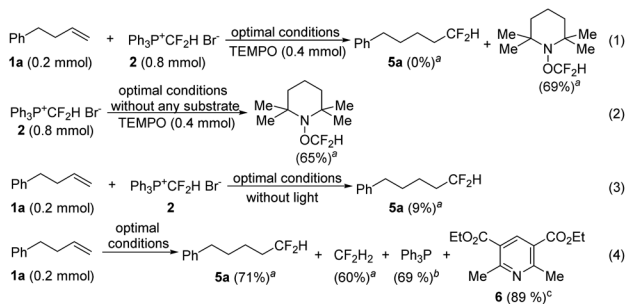
Scheme 3 Mechanistic investigations. a The yields were determined by ^{19}\text{F} NMR spectroscopy based on 1a (0.2 mmol); b isolated yield based on [\text{Ph}_3\text{P}^+\text{CF}_2\text{H}]\text{Br}^- ; c isolated yield based on the Hantzsch ester.
