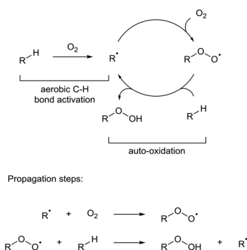
Scheme 1 General dioxygen-initiated autooxidation pathway.
