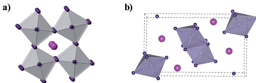
Fig. 6 (a) Crystal structure of B- \gamma -CsSnI 3 . B(b) Crystal structure of Y-CsSnI 3 . In these two images, the magenta spheres represent the Cs atoms, the purple spheres represent the I atoms, and the gray spheres represent the Sn atoms.
