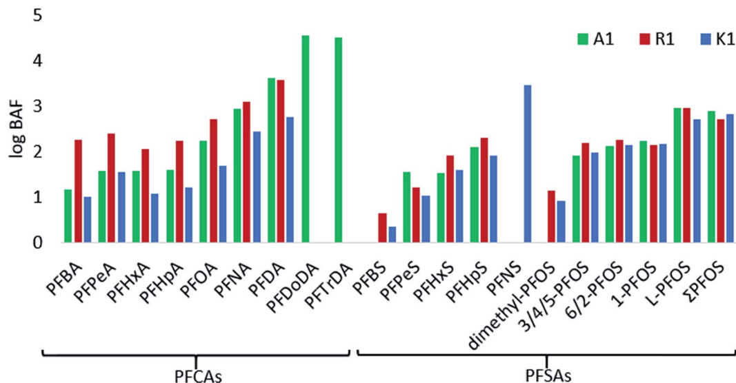
Fig. 4 The logarithmic bioaccumulation factor (BAF) on a wet weight basis ( \text{L kg}^{-1} ) of target PFCAs and PFSA/PFOS isomers, linear PFOS and \Sigma PFOS for sites A1, R1 and K1. The BAFs could not be determined for some PFASs and sites due to values below MDL.
