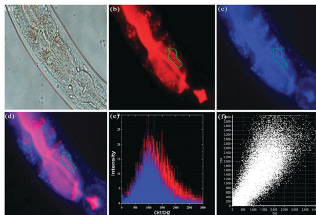
Fig. 91 Colocalization imaging of lysosomes in C. elegans . (a) Bright field image. (b) 500 \mu\text{M} AO incubated for 4 h at 20 ^{\circ}\text{C} (channel 2: \lambda_{\text{ex}} = 485 nm, \lambda_{\text{em}} = 510–550 nm). (c) 10.0 \mu\text{M} 57 with 300 \mu\text{M} of \text{H}_2\text{S} incubated for 30 min at 20 ^{\circ}\text{C} (channel 1: \lambda_{\text{ex}} = 385 nm, \lambda_{\text{em}} = 405–440 nm). (d) The merged image of channels 1 and 2. (e) The intensity profile of the regions of interest (ROI) across C. elegans . (f) The intensity correlation plot of 57 and AO. Copyright 2014 Royal Society of Chemistry.
