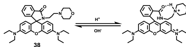
Scheme 28 Fluorescent probe 38 for pH.
