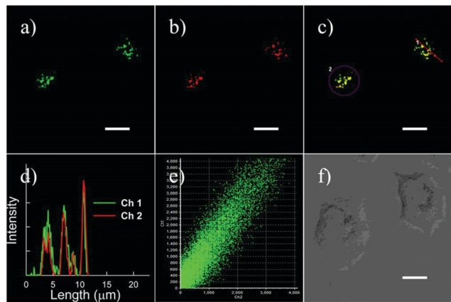
Fig. 88 Probe 56 colocalizes to the lysosome in HeLa cells. Cells were stained with (a) LysoTracker Green (1.0 \mu\text{M} , channel 1 (Ch1, green), \lambda_{\text{ex}} = 488 nm; \lambda_{\text{em}} = 505–530 nm) and (b) probe 56 (5.0 \mu\text{M} , channel 2 (Ch2, red), \lambda_{\text{ex}} = 515 nm; \lambda_{\text{em}} = 540–580 nm) with NaHS solution (50.0 \mu\text{M} ) for 60 min at 37 ^{\circ}\text{C} . (c) Overlay of parts (a) and (b). (d) Intensity profile of the linear region of interest (ROI 1) across the HeLa cell costained with LysoTracker Green and 56 . (e) Intensity scatter plot of Ch1 and Ch2 in ROI 2. (f) Bright-field images. Scale bar: 10 \mu\text{m} . Copyright 2014 American Chemical Society.
