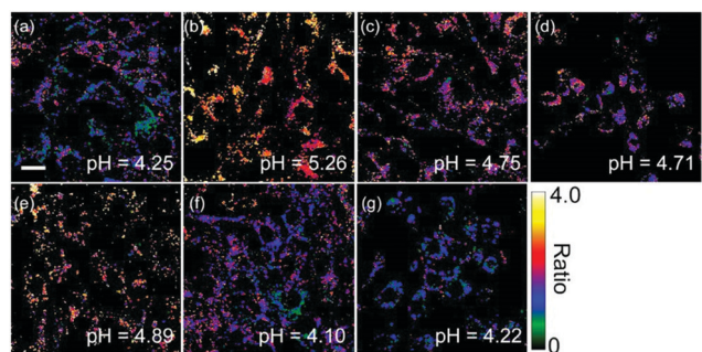
Fig. 45 Ratiometric imaging of NIH 3T3 cells. The cells were incubated with probe 29 (2 \mu M) at 37 ^\circ\text{C} for 30 min and then treated with (a) PBS at 25 ^\circ\text{C} for 3 min, (b) 10 mM \text{NH}_4\text{Cl} at 25 ^\circ\text{C} for 1 min, (c) 50 \mu M chloroquine at 25 ^\circ\text{C} for 3 min, (d) 100 \mu M \text{H}_2\text{O}_2 at 25 ^\circ\text{C} for 30 min, (e) 100 \mu M \text{HClO} at 37 ^\circ\text{C} for 30 min. The cells were pretreated with (f) 100 \mu M NEM and (g) 500 \mu M NAC at 37 ^\circ\text{C} for 30 min then incubated with 29 (2 \mu M) for further 30 min. Average pH values were measured from 10 cells in (a–g) and were calculated from the ratio ( F_{\text{green}}/F_{\text{red}} ) according to the intracellular calibration curve. Scale bar: 20 \mu m, ratio bar: 0–4. Copyright 2013 American Chemical Society.
