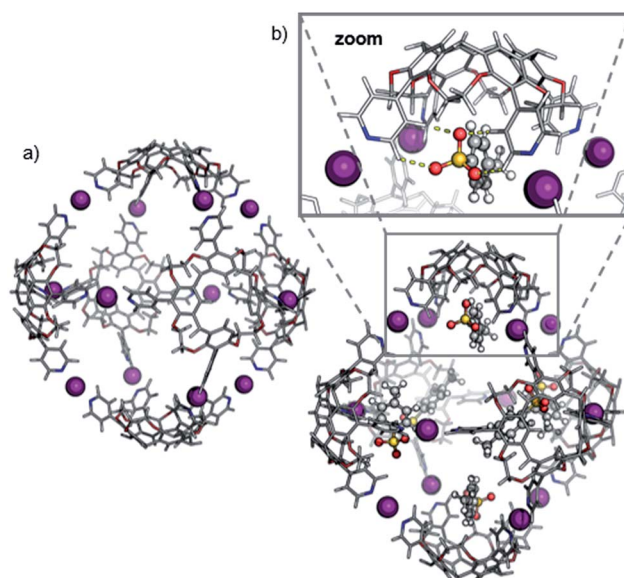
Fig. 4 Geometry-optimized structure of the hexameric halogen-bonded capsule 2 (a) in the absence of tosylate ions ( [6\cdot C_H + 12I]^{12+} ) and (b) with six tosylate anions ( [6\cdot C_H + 12I + 6\cdot OTs]^{6+} ). The n -hexyl chains are omitted for clarity. Inset: binding situation of a tosylate counterion.
