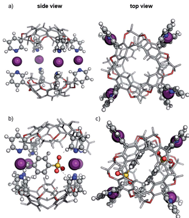
Fig. 2 Geometry-optimized structures of dimeric halogen-bonded capsule 1 (a) in the absence of tosylate counterions ( [2\cdot C_D + 4I]^{4+} ; side and top view); (b) with one tosylate inside the cavity ( [2\cdot C_D + 4I + OTs]^{3+} ), [C_{aryl}-H\cdots O^-] interactions are marked with dotted lines; (c) with two tosylates inside the cavity ( [2\cdot C_D + 4I + 2OTs]^{2+} ). PBE0/def2-SVP was used for I^+ , pyridines and tosylates (ball-and-stick representation); AM1 for the cavitand scaffold (stick representation). For clarity, the n -hexyl chains are omitted in the images.
