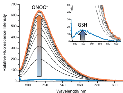
Fig. 2 Fluorescence spectra of GSH-PF3 (0.5 \mu\text{M} ) with addition of GSH (200 \mu\text{M} ), 10 min wait (inset), then addition of ONOO - (0–10 \mu\text{M} ) in buffer solution [52 wt% methanol] (pH = 8.21 at 25 ^{\circ}\text{C} ). Fluorescence intensities were measured with \lambda_{\text{ex}} = 488 \text{ nm} with slit widths ex slit: 5 nm and em slit: 2.5 nm.
