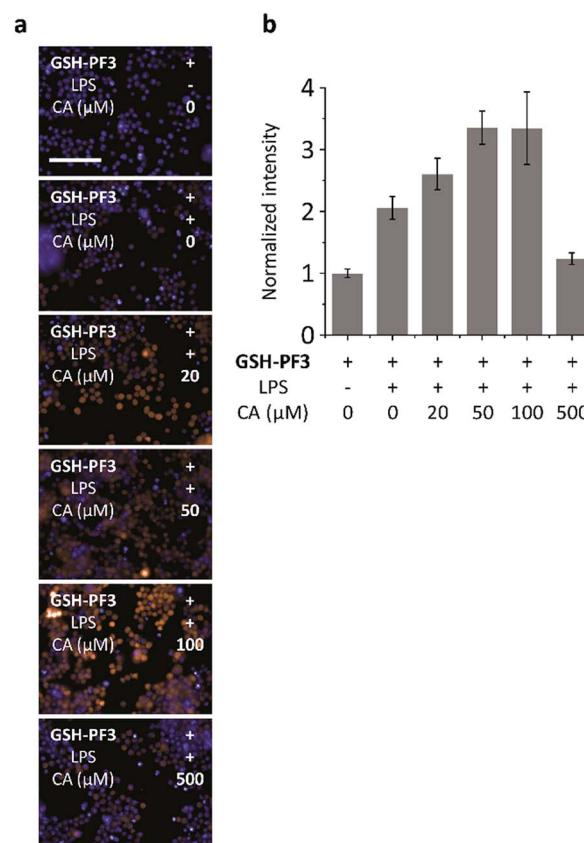
Fig. 4 Fluorescence imaging (a) and quantification (b) of RAW264.7 cells with GSH-PF3 (10 \mu\text{M} ) in the absence and presence of LPS (1 \mu\text{g mL}^{-1} ), which elicits ONOO - and increasing caffeic acid (CA, a drug that elicits endogenous GSH to quench ONOO - ). Excitation channel = 460–490 nm, emission channel filtered = 530–590 nm. Cell nuclei were stained with Hoechst 33342. Scale bar = 100 \mu\text{m} . Error bars represent SD.
