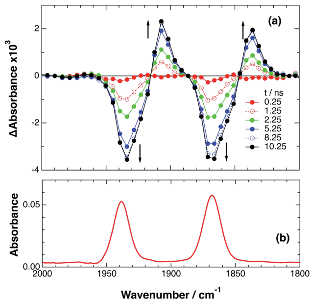
Fig. 6 (a) TRIR spectra (ps-system) recorded after 532 nm excitation of \text{RuRe(FPh)} (0.2 mM) in a \text{DMF-TEOA} (5 : 1 v/v) solution containing BIH (0.3 M), (b) FT-IR spectrum of \text{RuRe(FPh)} in a \text{DMF-TEOA} (5 : 1 v/v) solution.
