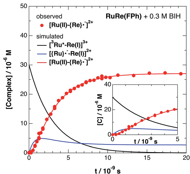
Fig. 7 Time profile of [\text{Ru(II)}-\{\text{Re}\}]^{2+} (●) in the ps-TRIR measurement of \text{RuRe(FPh)} in the presence of 0.3 M BIH in an argon-saturated \text{DMF-TEOA} (5 : 1 v/v) solution after 532 nm excitation. The kinetic simulation results for [^3\text{Ru}^*-\text{Re(I)}]^{3+} , [\{\text{Ru}\}^+-\text{Re(I)}]^{2+} , and [\text{Ru(II)}-\{\text{Re}\}]^{2+} are also shown (solid lines).
