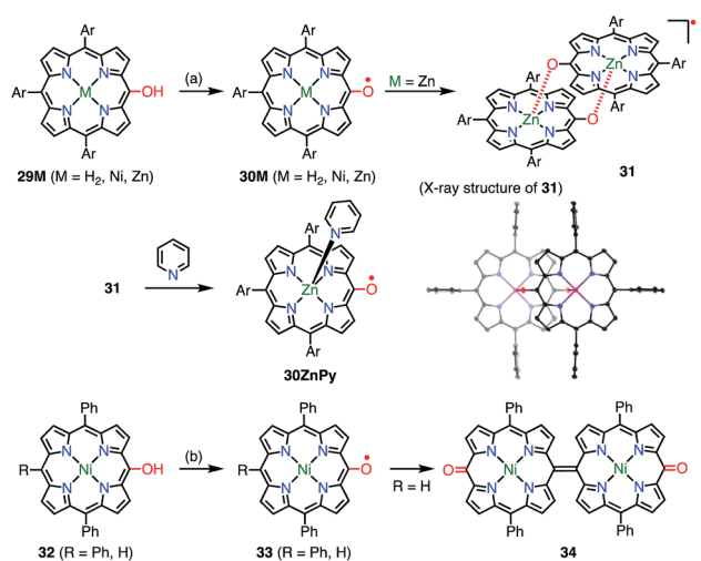
Fig. 11 10,15,20-Triarylporphyrin meso -oxy radicals. (a) 800 equiv. \text{PbO}_2 , \text{CH}_2\text{Cl}_2 , rt, 5 min, 86% for 30H 2 , 91% for 30Ni , 89% for 31 ; (b) aerobic oxidation for 33 , 7 equiv. DDQ, \text{CH}_2\text{Cl}_2 , rt, 30 min, 26% for 34 . Ar = 3,5-di- tert -butylphenyl. Hydrogen atoms and tert -butyl groups in the crystal structure of 31 were omitted for clarity.
