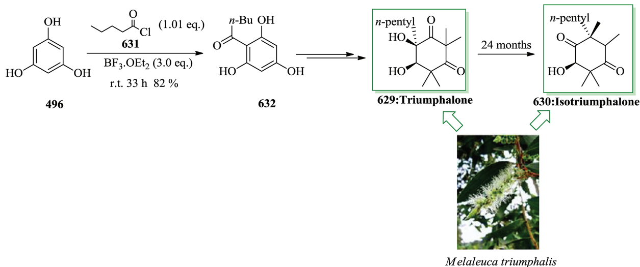
Scheme 136 Total synthesis of triumphalone 629 and isotriumphalone 630 .
