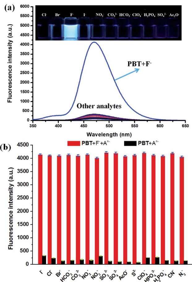
Fig. 6 (a) Fluorescence spectra of PBT in the presence of various anions. [PBT] = 10 \mu M, [ An^- ] = 20 \mu M, in a mixture of THF and Tris buffer solution (pH 8.0), (1 : 9, v/v), \lambda_{ex} = 335 nm, \lambda_{em} = 470 nm. Inset: direct observation of fluorescence emission difference of the probe PBT (10 \mu M) under UV irradiation (365 nm) in the presence of different anions. Left to right: Cl^- , Br^- , I^- , F^- , NO_2^- , CO_3^{2-} , HCO_3^- , ClO_4^- , H_2PO_4^- , SO_4^{2-} and AcO^- . (b) The selectivity of PBT in the presence of various anions.
