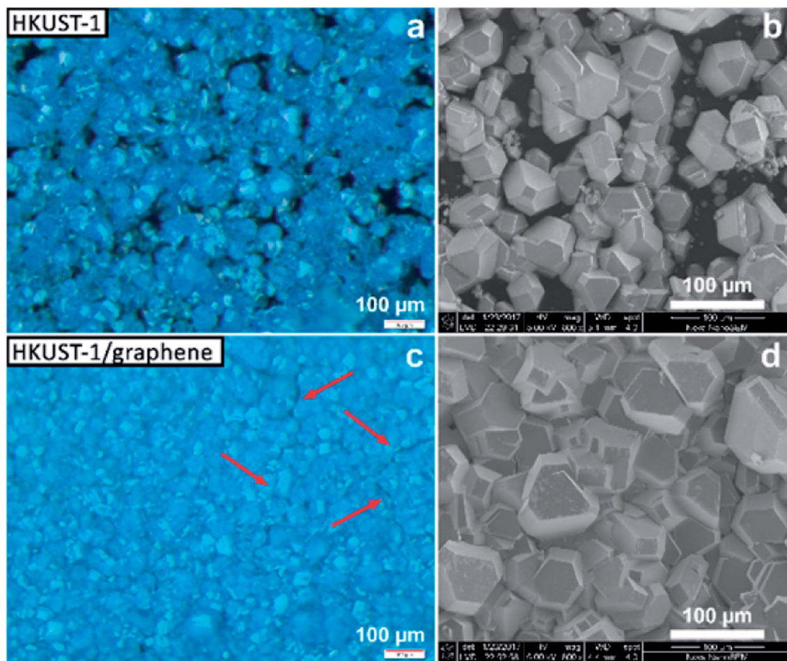
Fig. 2 Optical microscopy (left) and SEM (right) images of films of HKUST-1 (top) and HKUST-1/graphene (bottom). The HKUST-1 crystals form clusters on the surface of GC, leaving several areas uncoated, while the addition of graphene leads to complete coverage of the substrate. The red arrows indicate small cracks in the composites, possibly caused by mechanical stress in the films.
