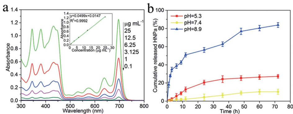
Fig. 4 (a) The standard absorption curves of HNPpa in ethanol at a wavelength of 698 nm by UV-vis spectra. (b) Percentage of cumulative released HNPpa (%) from MCGO drug carrier loading with HNPpa (MCGO-HNPpa) at 37 °C in phosphate buffer solution (pH = 5.3, 7.4 and 8.9) at different time points. The data points are based on triplicate samples.
