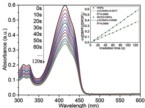
Fig. 5 Ultraviolet-visible absorption of DPBF after irradiation of MCGO-HNPpa, and first-order plots of the photodecomposition of DPBF photosensitized by HNPpa and MCGO-HNPpa with an equivalent concentration of HNPpa, monitoring the maximum absorption of DPBF at 415 nm.
