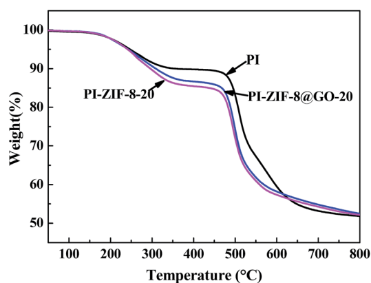
Fig. 10 TGA curves obtained for the unfilled PI, PI-ZIF-8@GO-20 and PI-ZIF-8-20 membranes.
