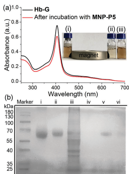
Fig. 3 (a) UV-vis spectra of Hb-G before (black line) and after (red line) being incubated with MNP-P5 . Inset photograph: Hb-G with (i) excess MNP , (ii) excess MNP-P5 , and (iii) no additive. (b) SDS-PAGE analysis of capturing the target protein from protein mixtures: native BSA (lane i), BSA-G (lane ii), BSA-G + IPEC-J2 cell lysate (lane iii); captured proteins recovered from MNP-P5 incubated in native BSA + IPEC-J2 cell lysate (lane iv), or BSA-G + IPEC-J2 cell lysate (lane v); captured proteins recovered from MNP incubated in BSA-G + IPEC-J2 cell lysate (lane vi).
